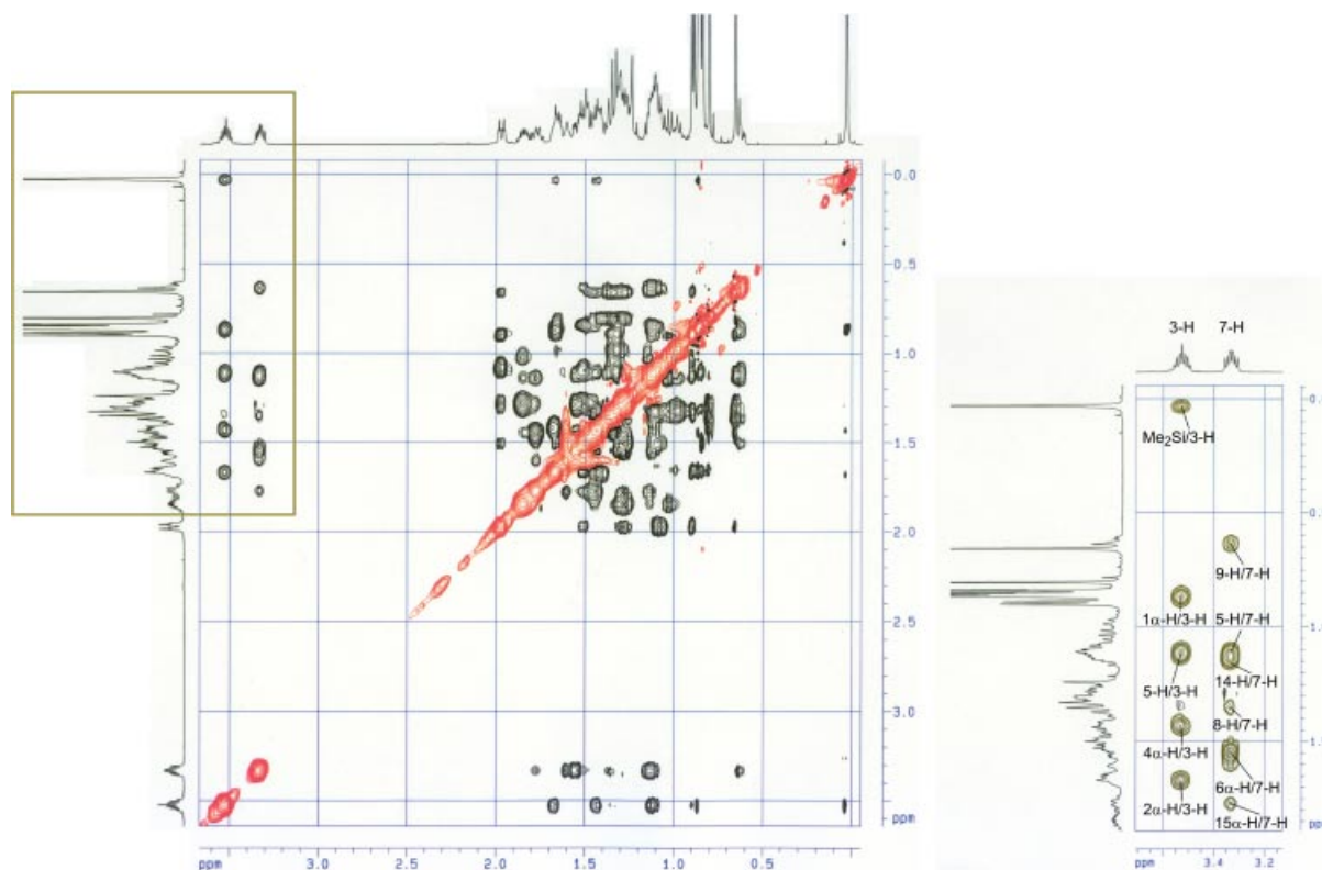
Figure 4. NOESY spectrum (500 MHz, CDCl 3 ) of 3 \beta -( tert -butyldimethylsilyloxy)-5 \alpha -cholestan-7 \beta -ol ( 23b ) and expansion of the region with characteristic signals.
