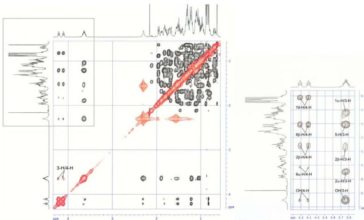
Figure 3. NOESY spectrum (500 MHz, \text{CDCl}_3 ) of 4α-fluoro-5α-cholestan-3β-ol ( 14b ) and expansion of the region with characteristic signals.
